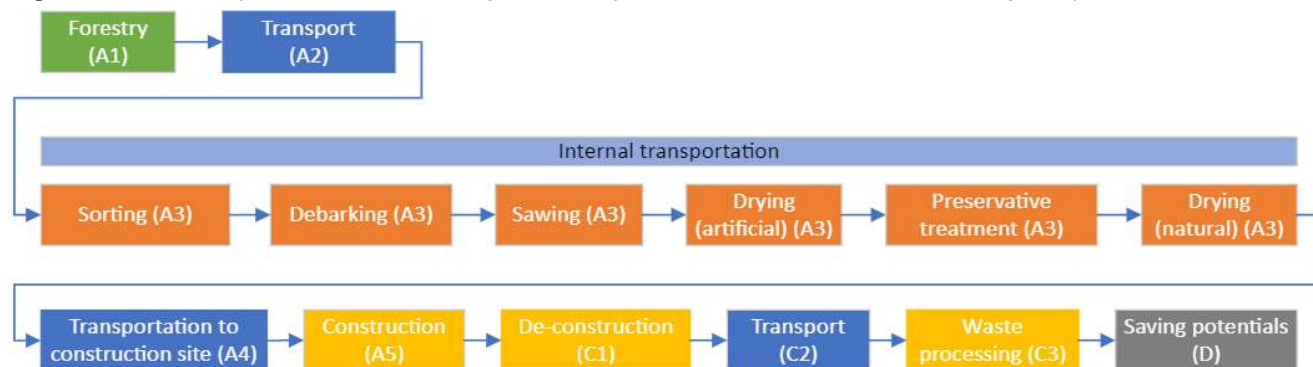
Figure 1 Declared product manufacturing and transport to a customer and the remaining lifecycle.
