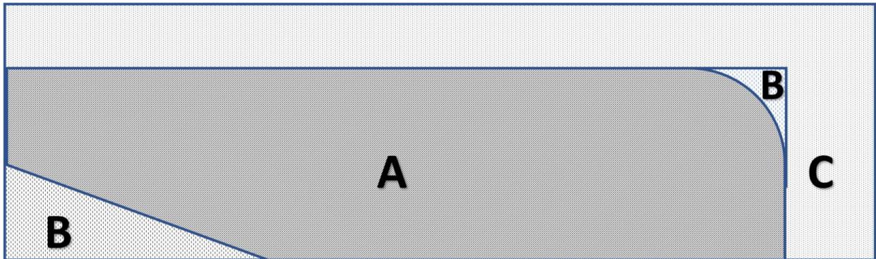
Figure 1: Measuring the volume of wood—illustration of a cross section of sawn timber. A = real measure / real dimensions of the finished product. B + C = planing allowance / shavings. A + B = actual size. A + B + C = nominal size / basic size. For a rectangular product, the real measure and the actual size are identical.
